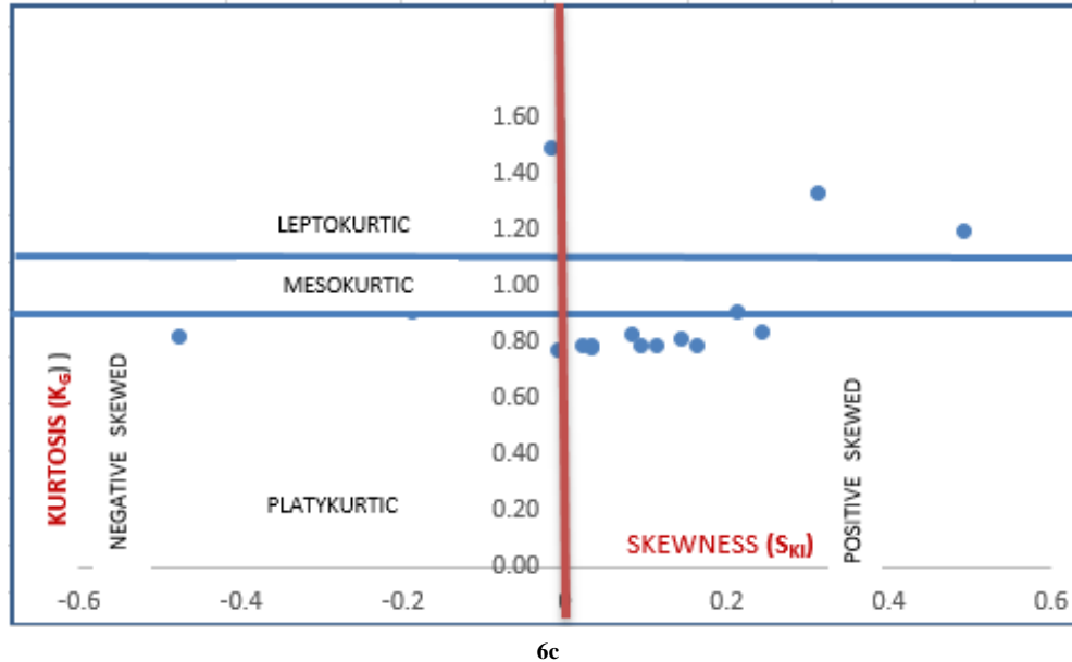
Figure 6: Bivariate plot of average values of grain size statistical parameters: (a) Sorting versus Grain size [4]. (b) Skewness against Grain size (c) Kurtosis versus Skewness.
