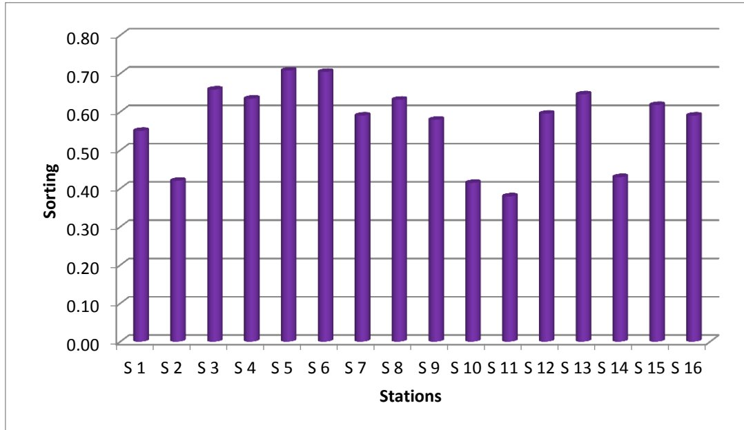
Figure 3. Distribution of grain size uniformity (Sorting) from study station
