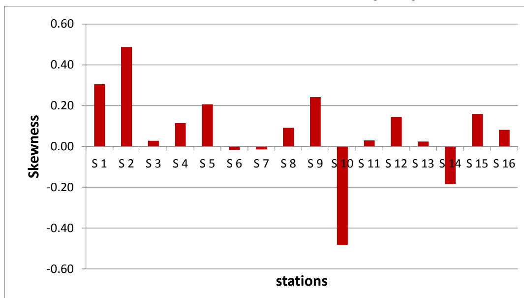
Figure 4. Skewness distribution from the study area
