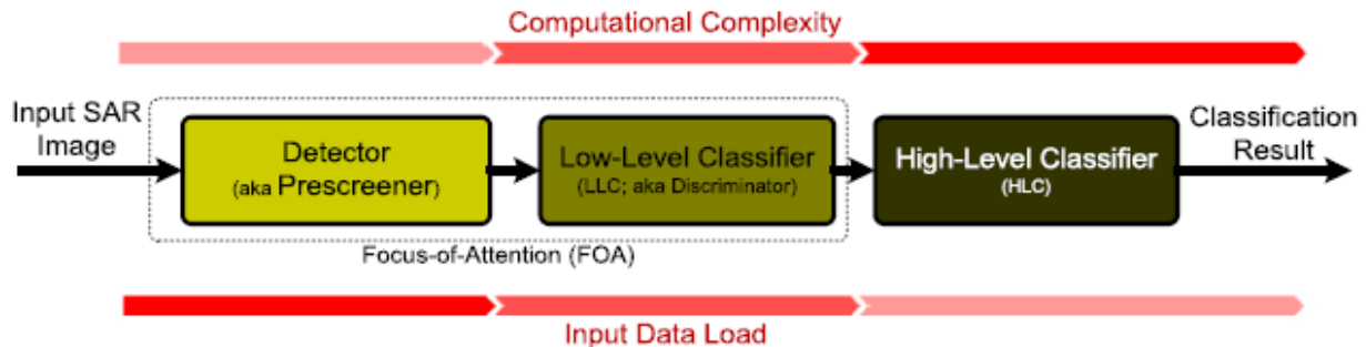
Figure 1 The Basic Structure of SAR-ATR end to end System
