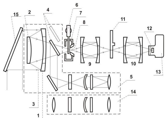
Fig. 1. Optical scheme of OMU.
