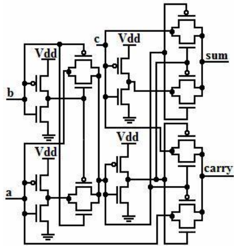
Fig. 3 Transmission Gate Full Adder [8]
