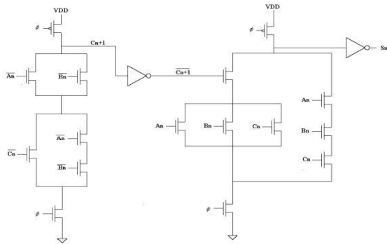
Fig. 4 Domino Logic Full Adder
