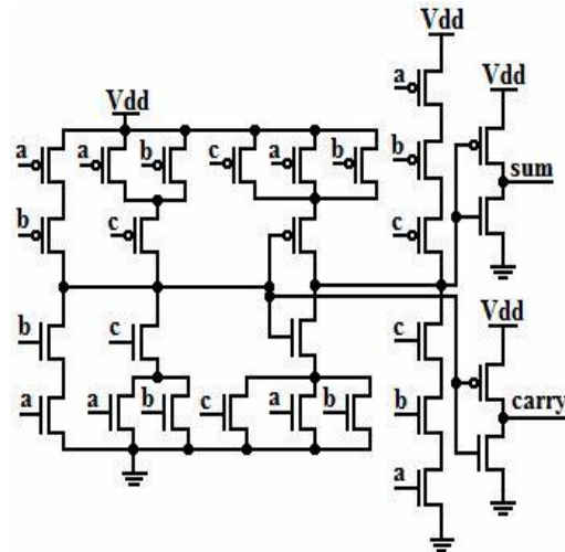
Fig. 1 CMOS Full Adder [8]
