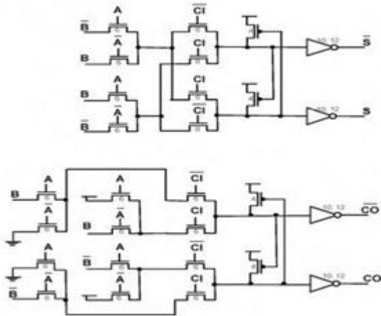
Fig. 2 CPL Full Adder Logic [3]
