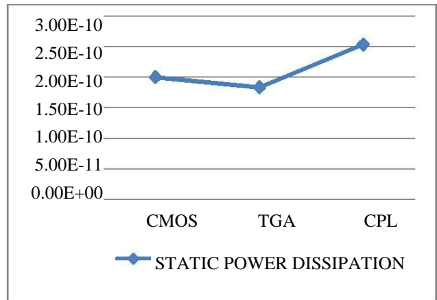
Fig. (b) Static Power Dissipation
