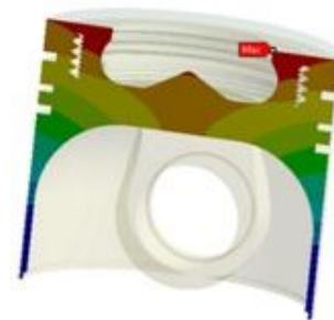
Fig5: Temperature contour
