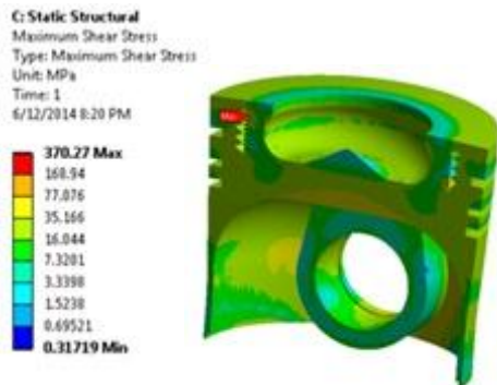
Fig8: Shear stress plot.
