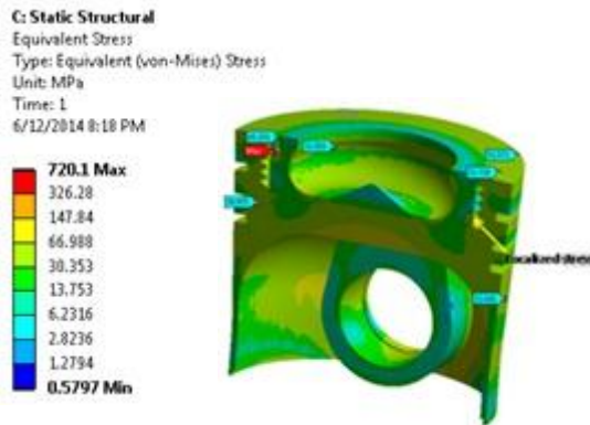
Fig 7: Von-mises plot.
