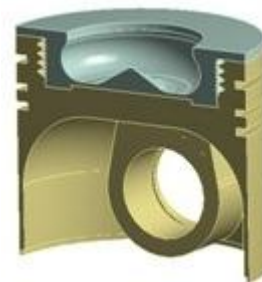
Fig 1: Sectional view of Modified Piston.
