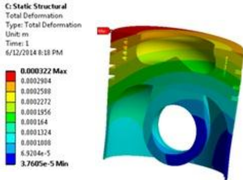
Fig 6: Displacement plot
