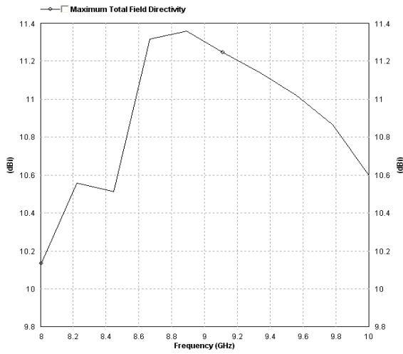
Total Field Directivity vs. Frequency
