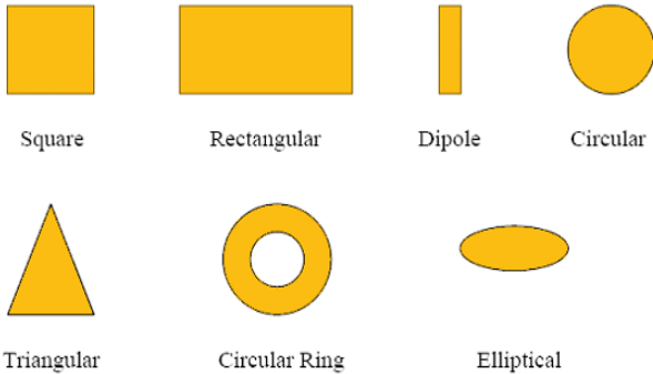
Fig. 1.1(a) Common shapes of micro strip patch elements
