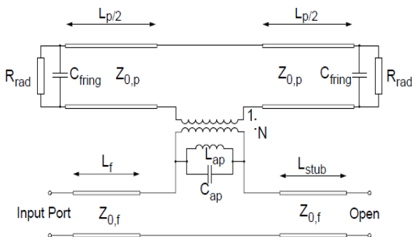
Fig. Equivalent circuit for an aperture-coupled micro-strip antenna
