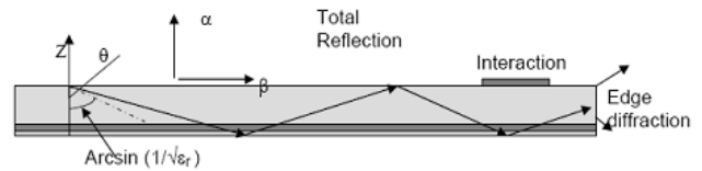
Figure 1.2. Surface waves
