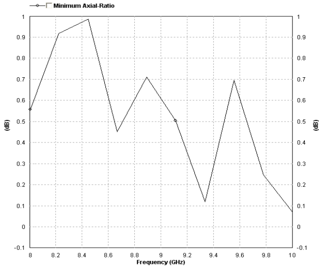
Axial-Ratio Vs. Frequency
