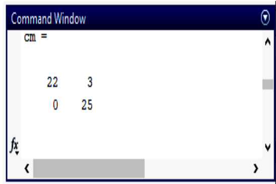
Figure 4: Confusion matrix
