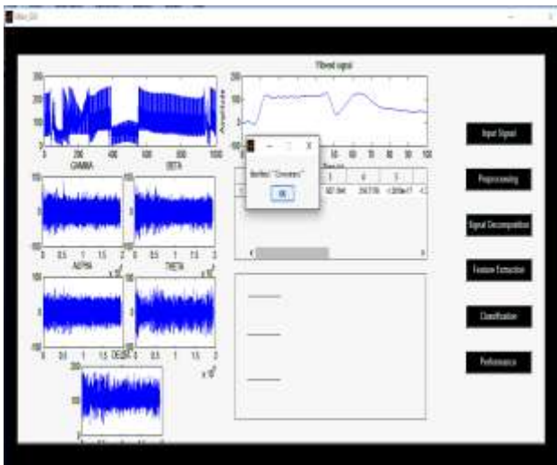
Figure 2: Classification
