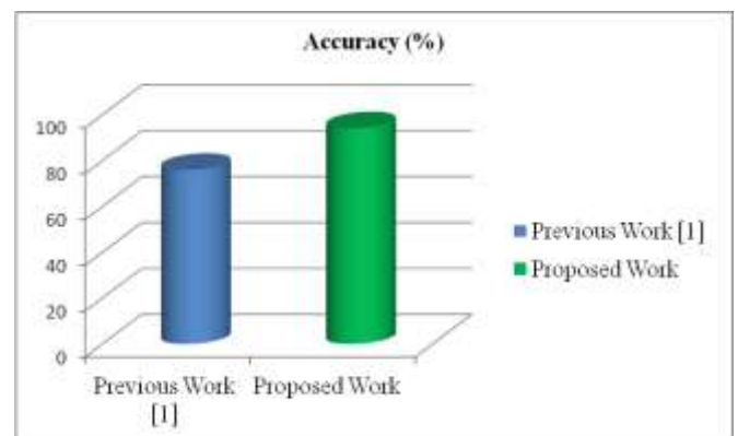
Figure 5: Comparison accuracy
