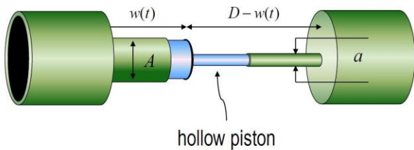
Fig. 5: Pipe model of a memristor.
