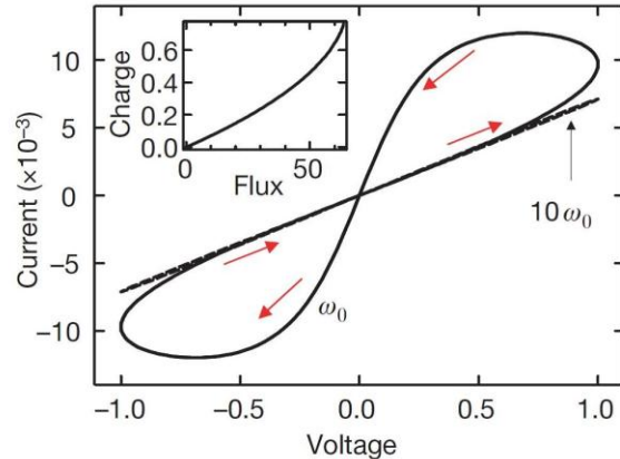
Fig. 6: Typical behavior of memristors.
