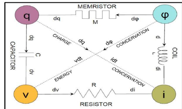
Fig. 2: Symmetry diagram showing the 6 distinct possible realizations based on the four circuit variables. Courtesy of C.
