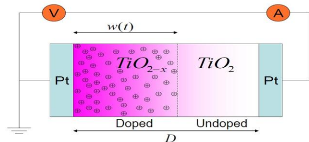
Fig. 4: Cross-section of the first HP TiO_2 -memristor consisting of a high conductive (doped) and a low conductive (undoped) part placed in between two platinum electrodes. The boundary between the 2 elements is dynamic and is affected back and forth by the passing charge carriers. The parameter w(t) is a mathematic variable that describes the position of this boundary. Courtesy of C. Lütken.
