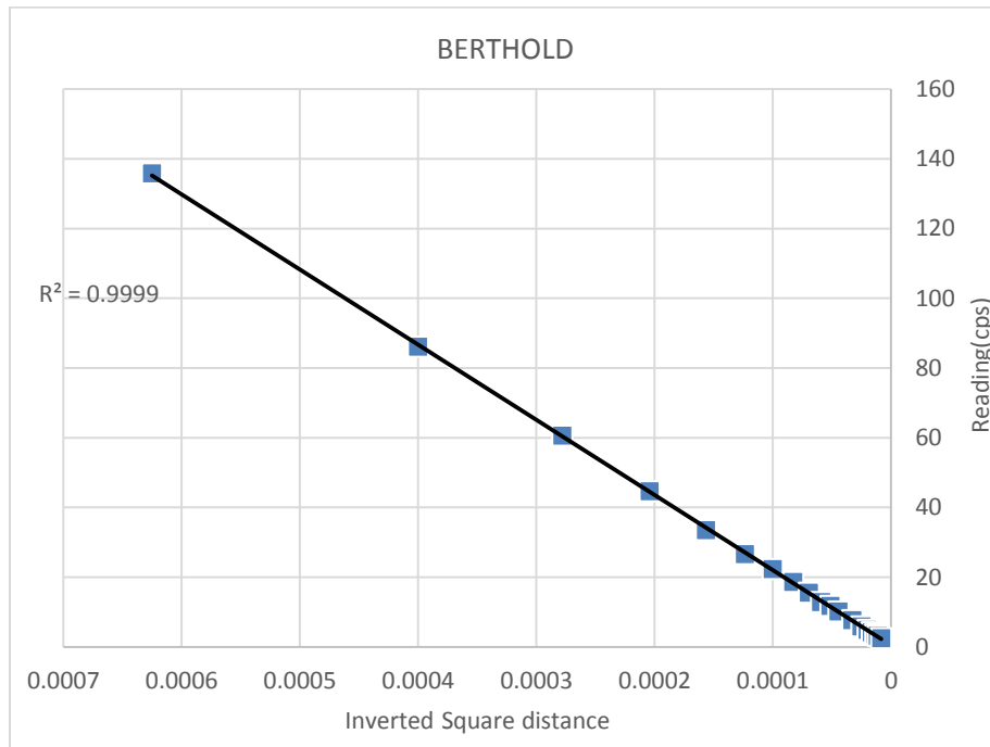
Fig. 4: Relation between the Berthold measurement and inverted square distance.
