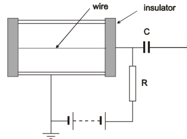
Fig. 1: Schematic diagram of detection of radiation.
