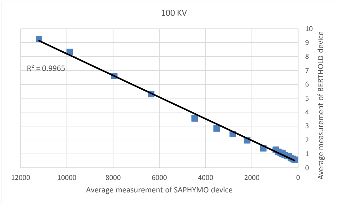
Fig (6) Relation between the Saphymo and Berthold measurement at different intensities (100 KV)
