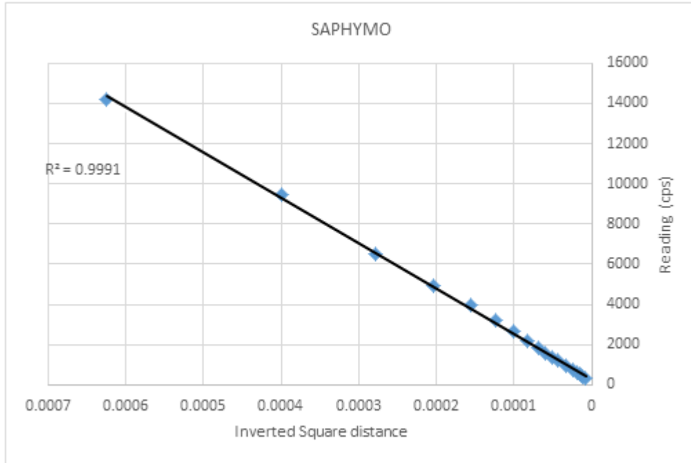
Fig. 3: Relation between the Saphymo measurement and inverted square distance.
