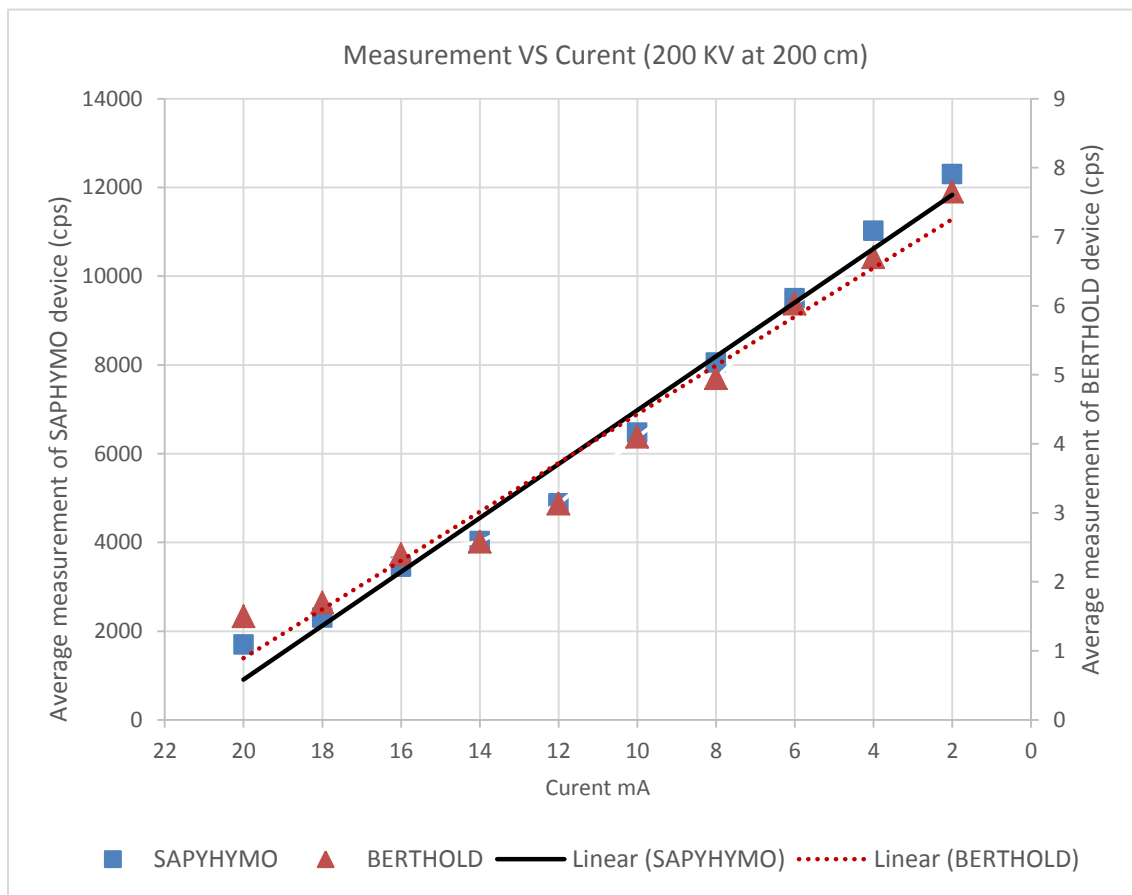
Fig. 5: Relation between the Saphymo and Berthold measurement and the current.
