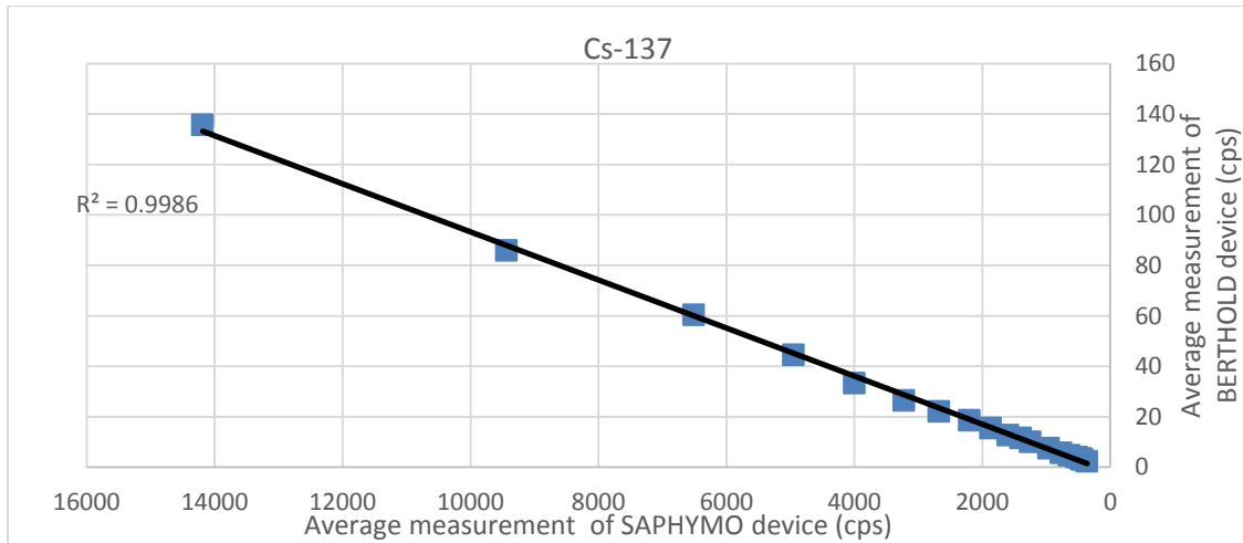
Fig. 8: Relation between the Saphymo and Berthold measurement at different intensities (Cs-137).
