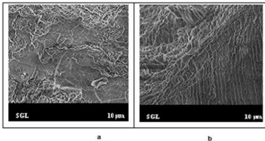
Figure 3. Microanalysis of deteriorated food surfaces at the time of: (a) summer and (b) winter in the interior of an industrial plant in Mexicali (2011) 10 X.
