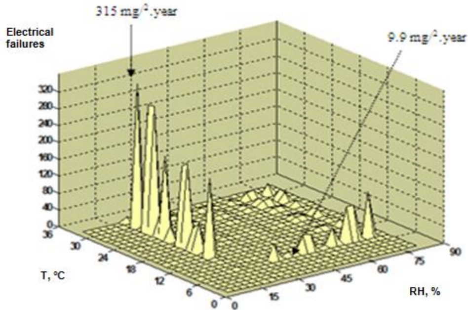
Figure 14 Correlation of electrical failures and climatic factors of an axial machine in summer (2016-2017)
