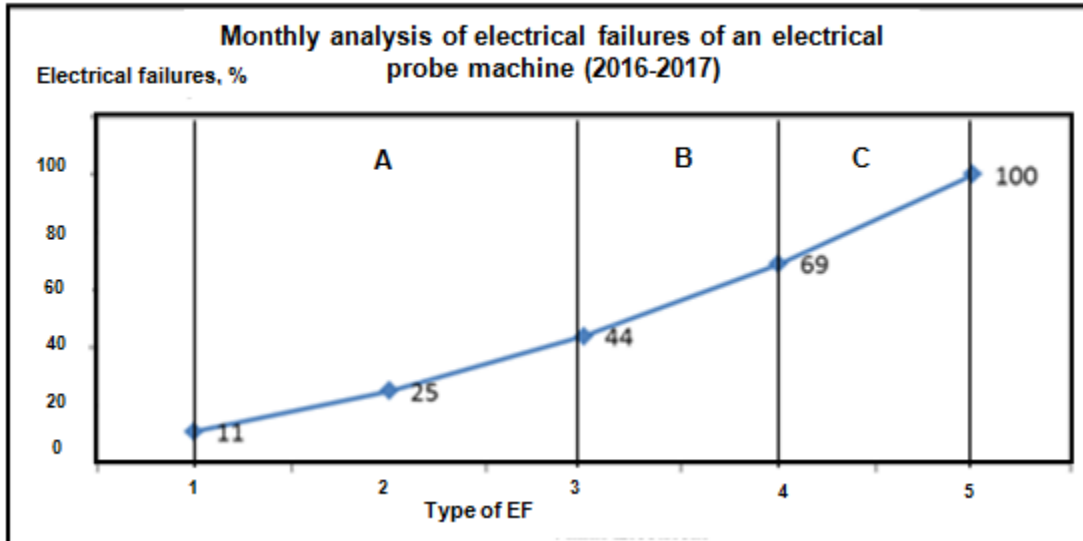
Figure 12 Monthly evaluation of electrical failures generated in a electrical probe machine (2016-2017)
