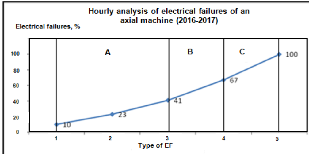
Figure 1 Hourly evaluation of electrical failures generated in an axial machine (2016-2017)
