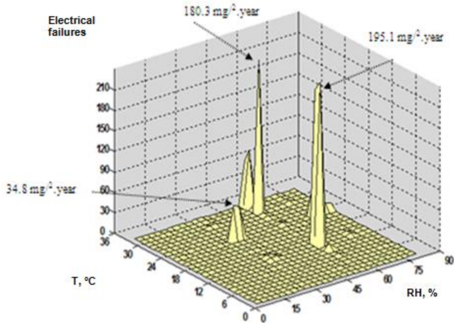
Figure 13 Correlation of electrical failures and climatic factors of an axial machine in winter (2016-2017)
